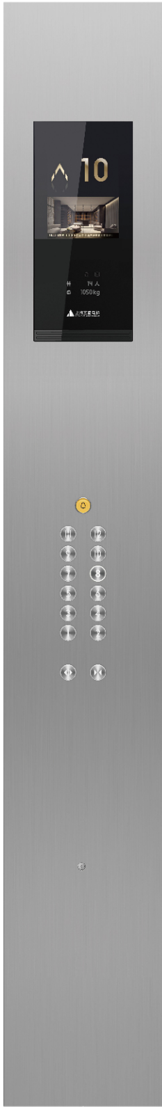
ZCB-T711 (Primary) ZCB-T761(Auxiliary) 10.4" TFT LCD, black gold interface (EMIDS) Resolution: 1024×768 The buttons are exchangeable. (Remark 9) The figure shown is A11 button. (Configurable when front wall≥250)
